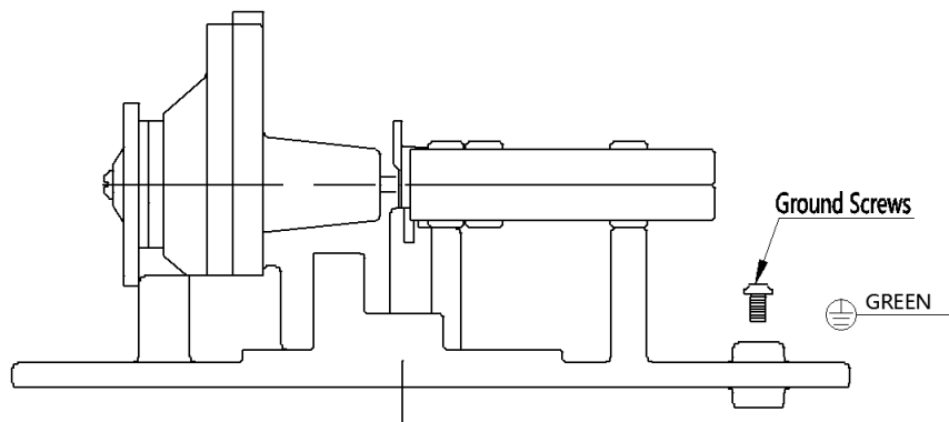
Fig.5 Ground screw
