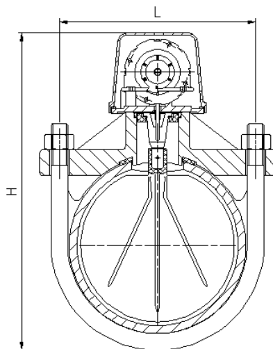
Fig.1 Mounting dimensions
