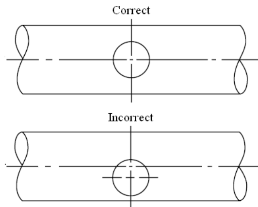
Fig.2 Mounting hole location
