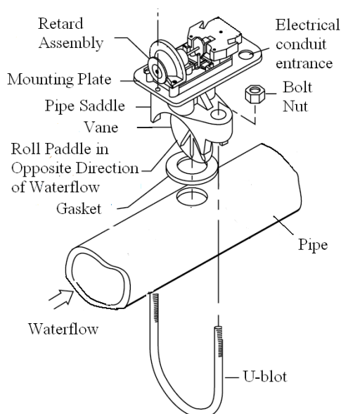
Fig.3 Assembly diagram
