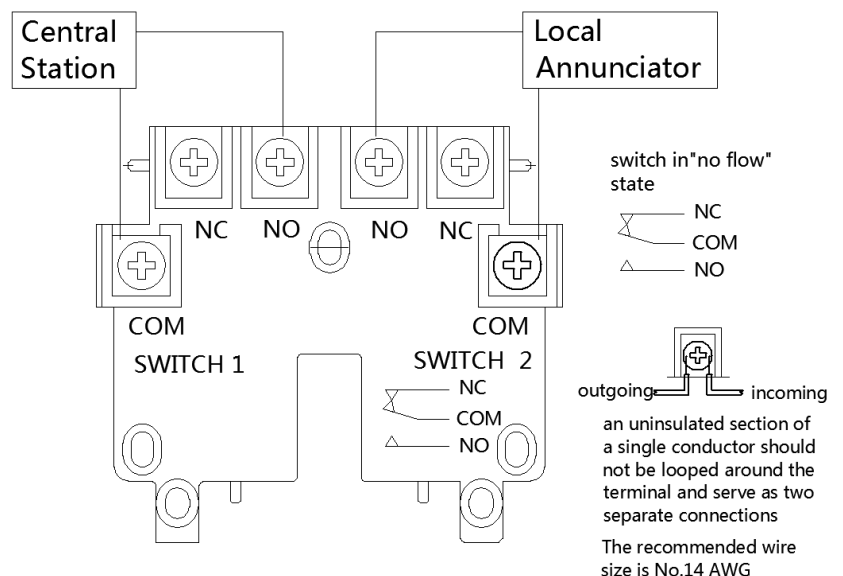
Fig.4 Typical electrical connections
